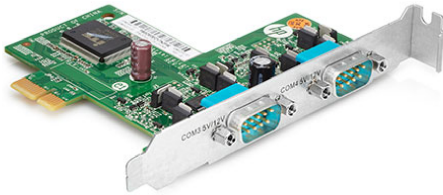
HP RS232-card for HP rp5800 #QP906AA
